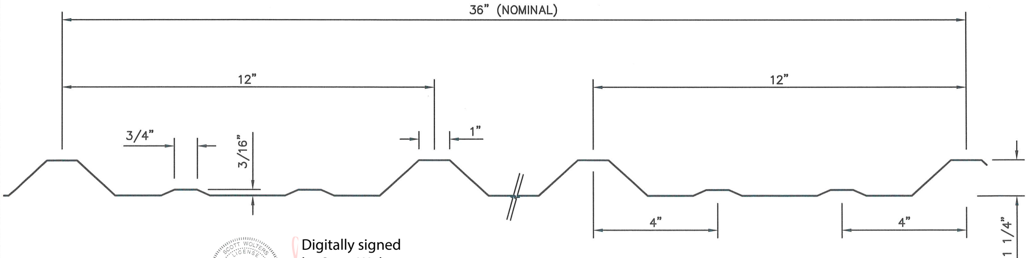
PANEL PROFILE
